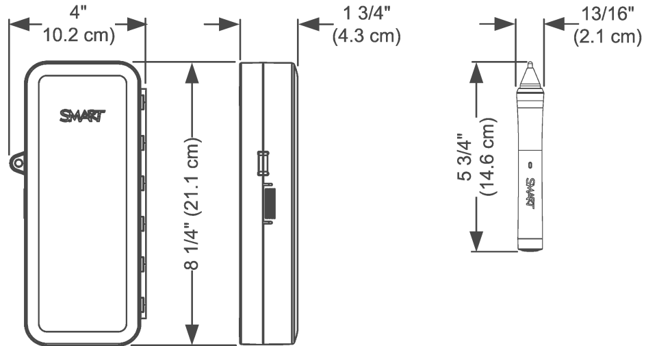
Interactive pen
