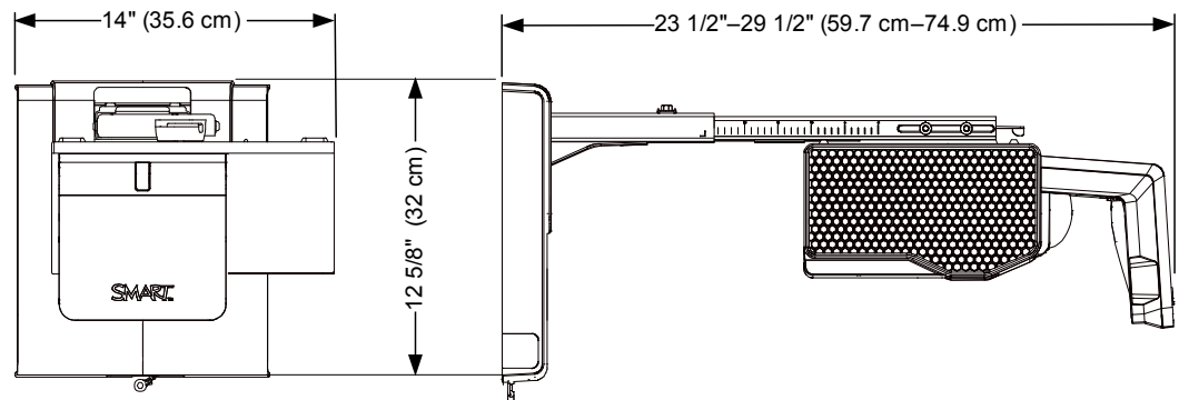
Interactive projector front view
